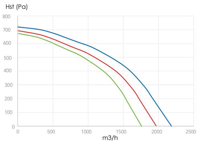
FVDA ACUSTIC 315
