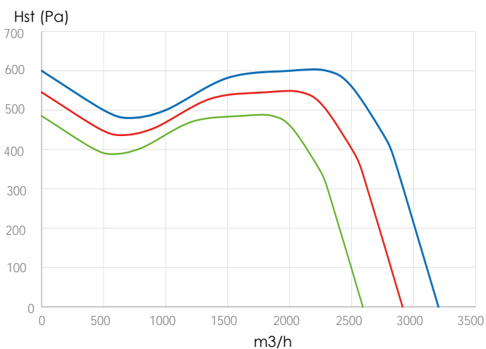
FVDA ACUSTIC 400
