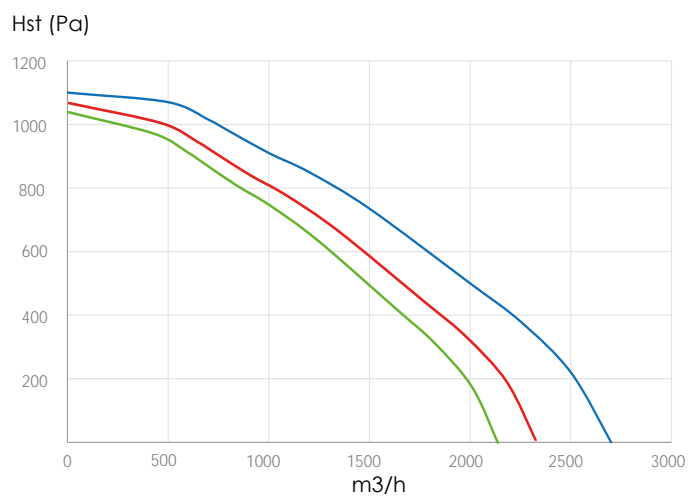
FVDA ACUSTIC 350
