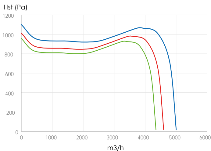
FVDA ACUSTIC 450
